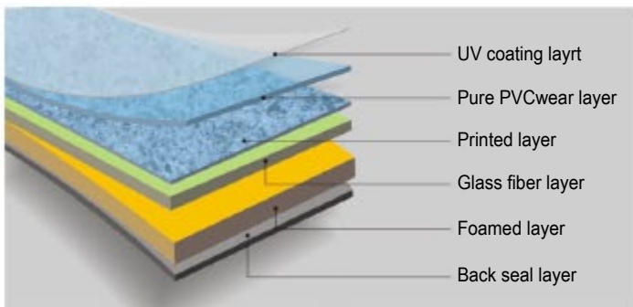
Product structure
