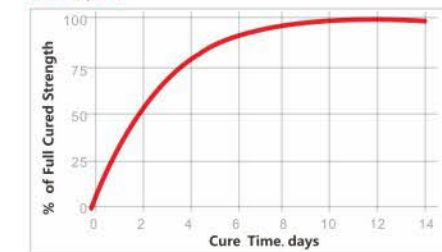
Cure Speed
