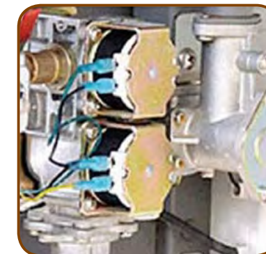
Double electromagnetic distribution control
